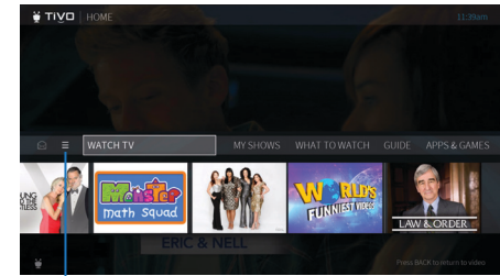
Settings menu
